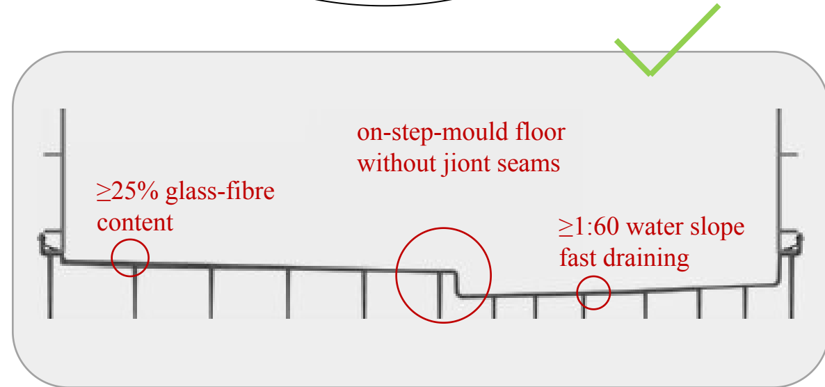
Joint 2-piece floor
